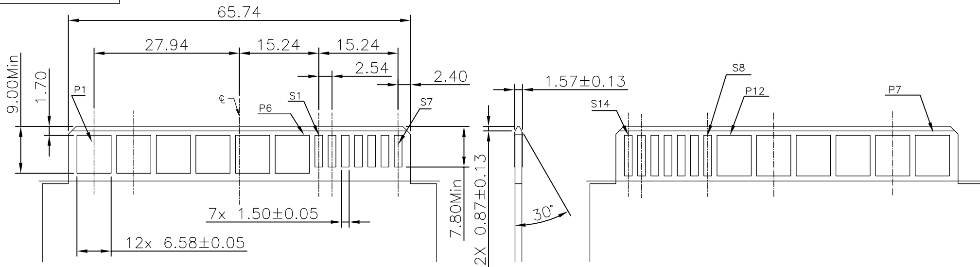
RECOMMENDED EDGE CARD LAYOUT THICKNESS IS 1.57±0.13MM; DIMENSION TOLERANCE: ±0.05MM
