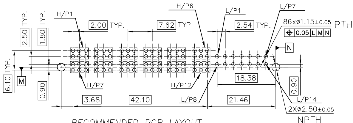
RECOMMENDED PCB LAYOUT DIMENSION TOLERANCE: ±0.05MM
