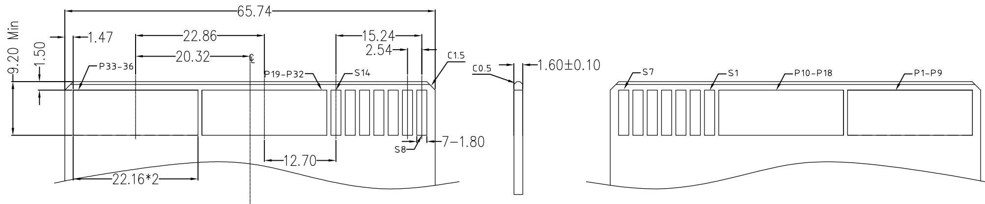
RECOMMENDED EDGE CARD LAYOUT (TOP VIEW) THICKNESS IS 1.57±0.13mm; DIMENSION TOLERANCE: ±0.05mm
