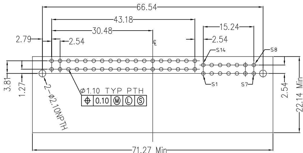
RECOMMENDED PCB LAYOUT (TOP VIEW) THICKNESS IS 2.00~2.4mm; DIMENSION TOLERANCE: ±0.05mm
