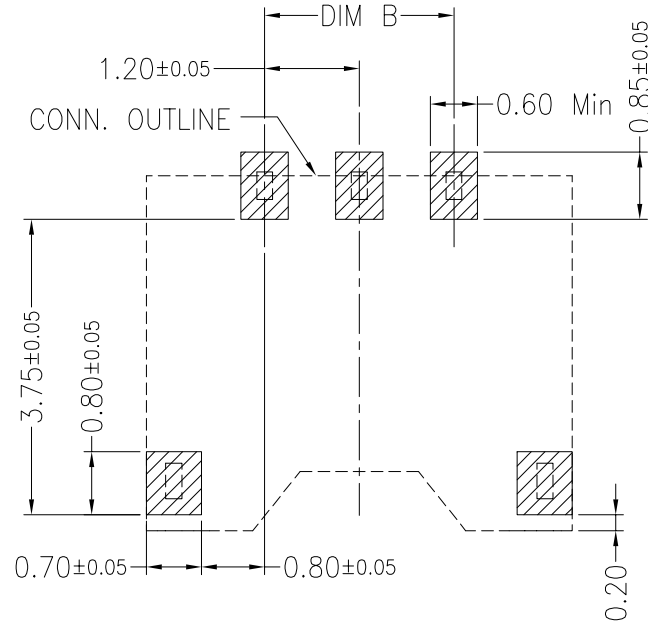
RECOMMENED PCB LAYOUT GENERAL TOLERANCE ±0.05
